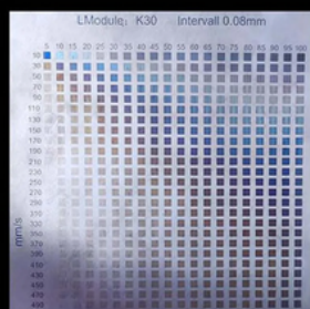
30W titanium engraving
